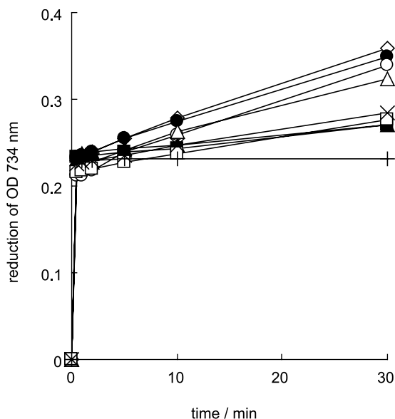
Figure 4. Time course of reduction of ABTS radical at OD 734 nm by C13aa ( \diamond ), T12 ( \bullet ), C12 ( \circ ), T13 ( \blacktriangle ), C13 ( \triangle ), T14 ( \blacksquare ), C14 ( \square ), CC ( \times ) and trolox ( + ). Concentration of tested compounds are 4\ \mu\text{M} except for CC and trolox ( 8\ \mu\text{M} ).
