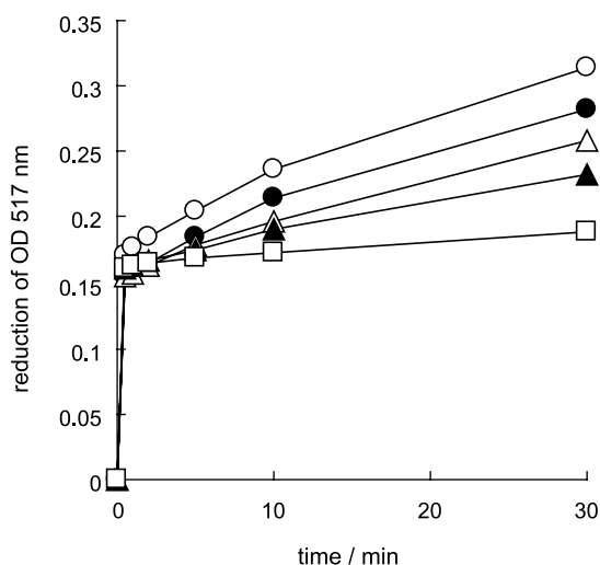
Figure 3. Time course of reduction of DPPH radical at OD 517 nm by T12 in aqueous ethanol. 60% water in ethanol ( \circ ), 40% water in ethanol ( \bullet ), 20% water in ethanol ( \triangle ), 10% water in ethanol ( \blacktriangle ) and ethanol ( \square ).
