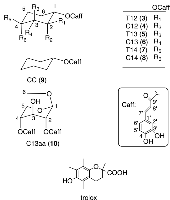
Figure 1. Structures of dicaffeoyloxycyclohexanes, 2,4-di- O -caffeoyl-1,6-anhydro- \beta -D-glucose, cyclohexyl caffeate and trolox.
