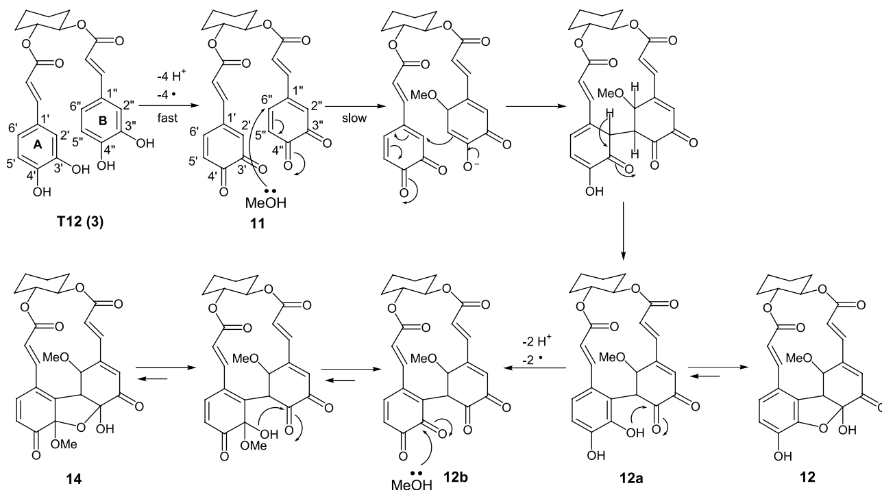
Figure 6. Plausible radical scavenging mechanism of T12 in water-methanol.
