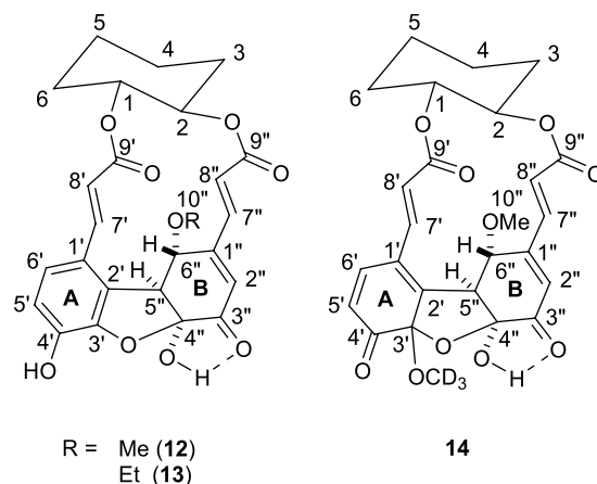
Figure 5. Structures of compounds 12 , 13 , and 14 .
