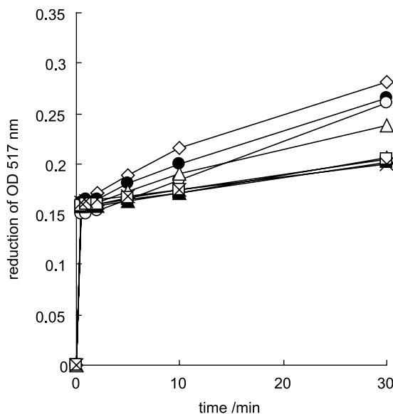
Figure 2. Time course of reduction of DPPH radical at OD 517 nm by C13aa ( \diamond ), T12 ( \bullet ), C12 ( \circ ), T13 ( \blacktriangle ), C13 ( \triangle ), T14 ( \blacksquare ), C14 ( \square ) and CC ( \times ). Concentrations of tested compounds are 4 \mu M except for CC (8 \mu M).
